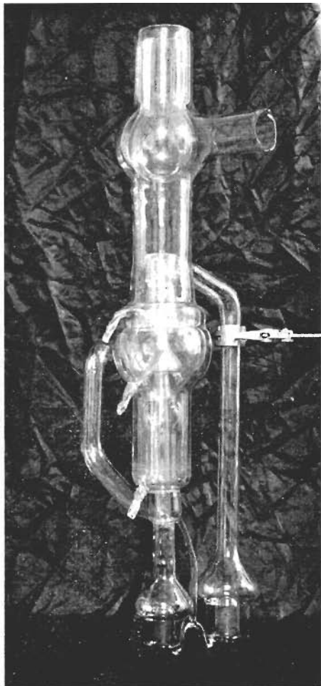
Fig. 22 A Two-stage annular jet mercury diffusion pump (Gray and Yorke)
