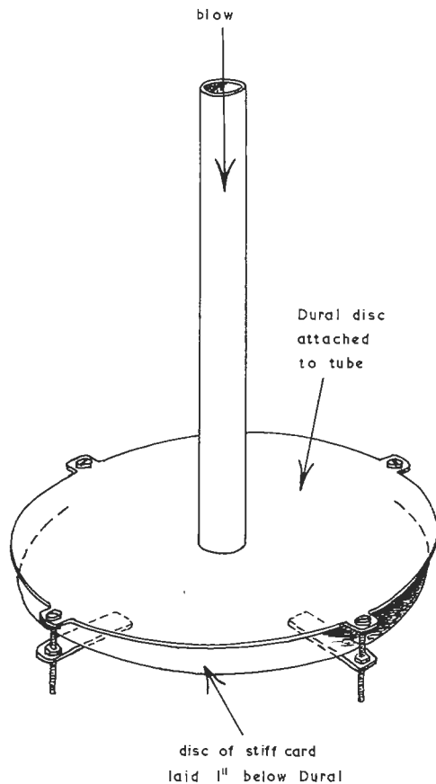
Fig. 14 Experiment to show that the density of a gas is a function of its velocity
