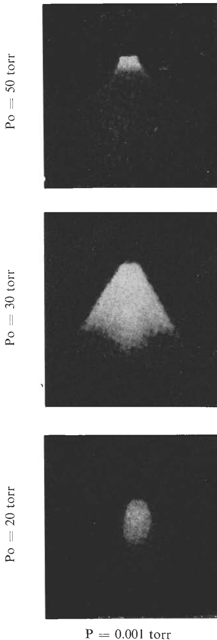
Fig. 16 Mercury vapour jet at three boiler pressures p_0 . Air pressure p surrounds the jet (Nöller 1955)
