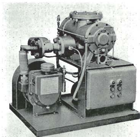
Fig. 12 Turbo-molecular pumping system (Welch Scientific Company)
