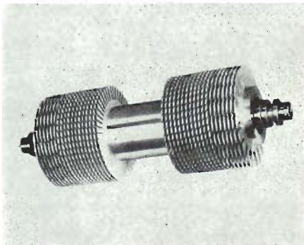
Fig. 13 Molecular pump rotor (Arthur Pfeiffer GmbH)
