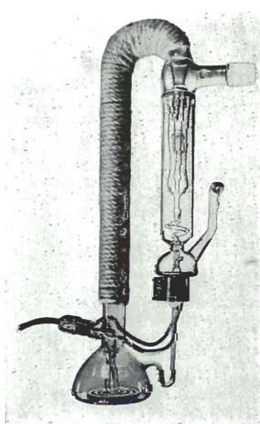
Fig. 10 Three-stage mercury vapour pump (Jenaer Glaswerk Schott and Gen., Model 3Q6)
