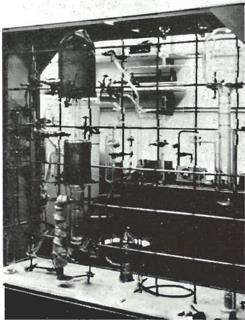
Fig. 3 Apparatus for measuring the speed of diffusion pumps (Courtesy of J. C. Snaith)
