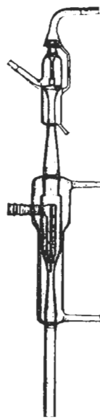
Fig. 11 Steam ejector pump (Leybold-Heraeus GMBH, Model WDS)
